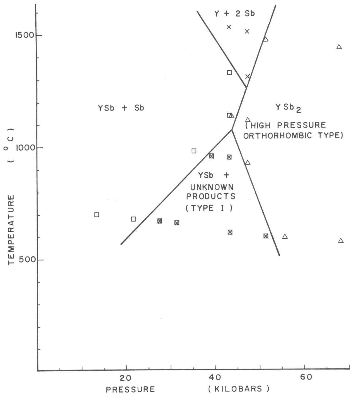
Fig 11.--Y + 2 Sb Reaction Product Diagram.
